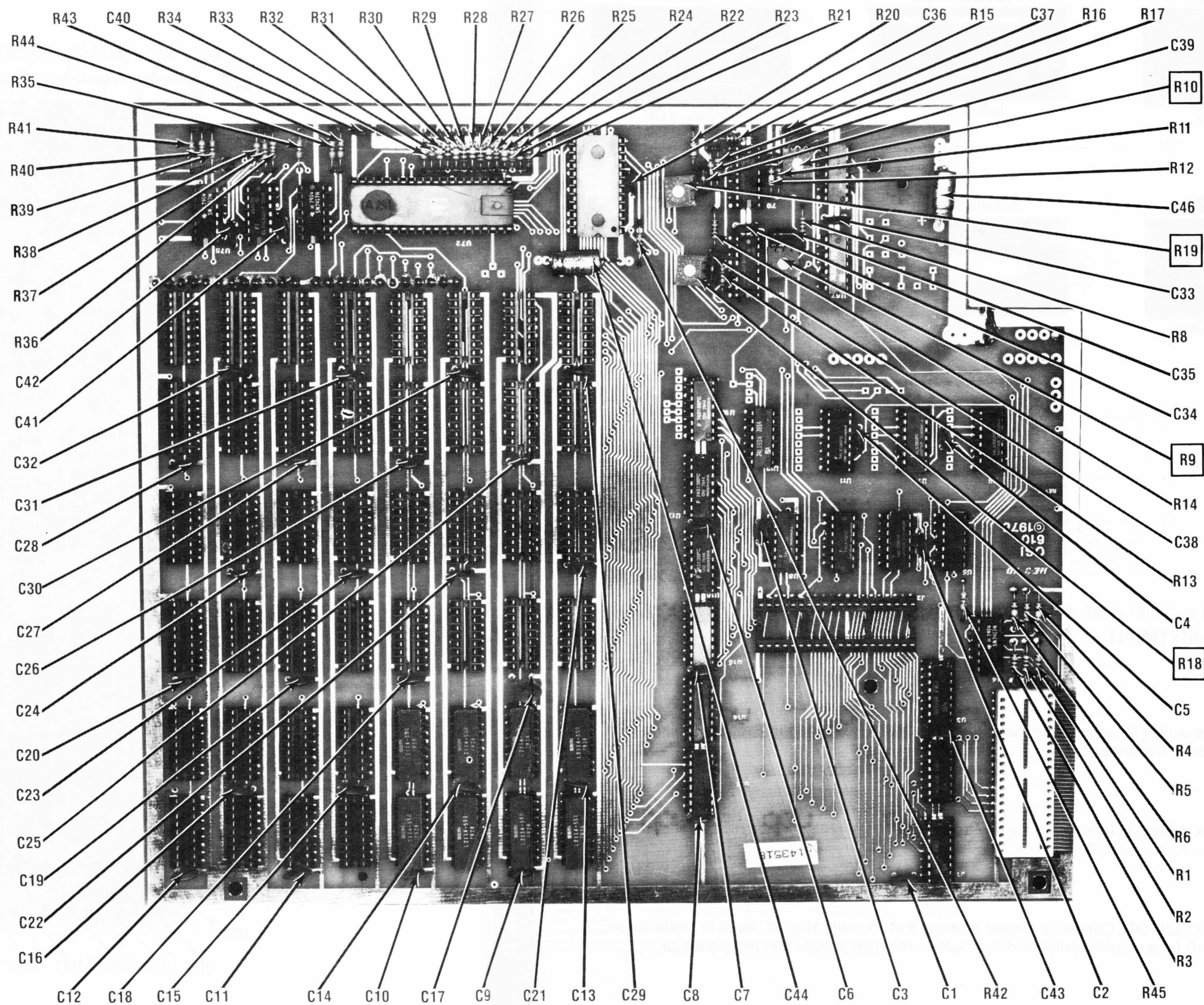
610 BOARD
